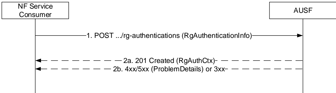
Figure 5.2.2.4-1: Authentication for FN-RG
