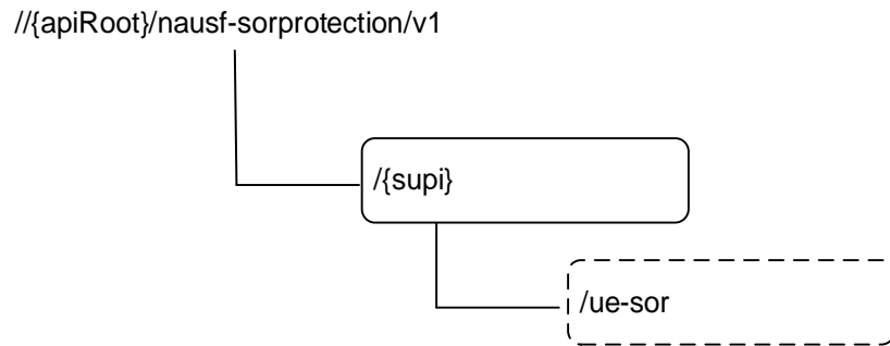
Figure 6.2.3.1-1: Resource URI structure of the SoRProtection API
