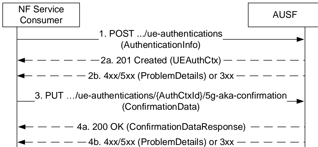
Figure 5.2.2.2.2-1: 5G AKA
