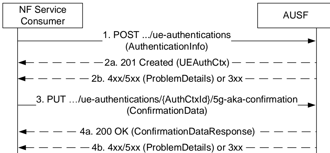
Figure 5.2.2.2-1: 5G AKA
