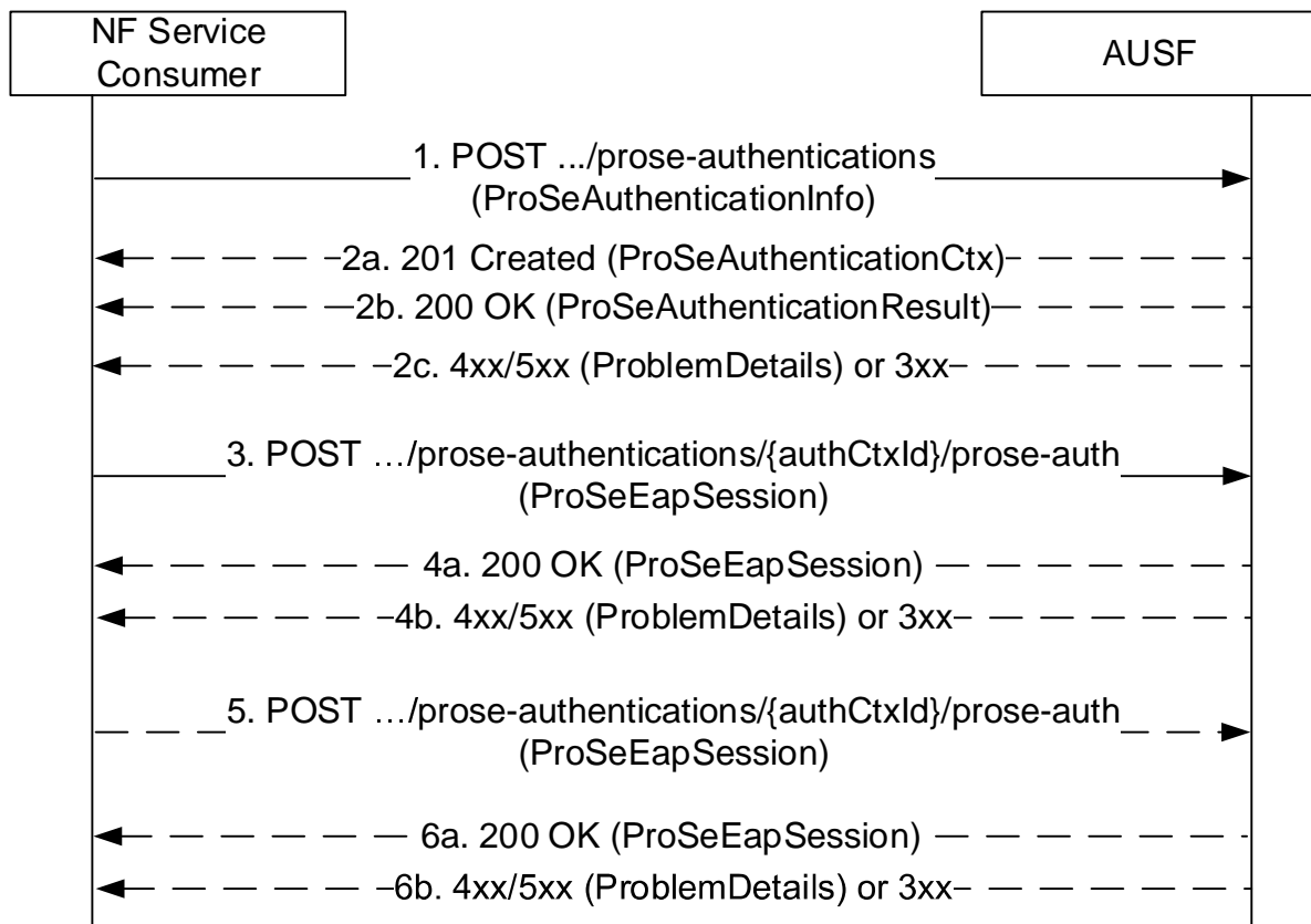
Figure 5.2.2.4.1-1: ProSe Authentication
