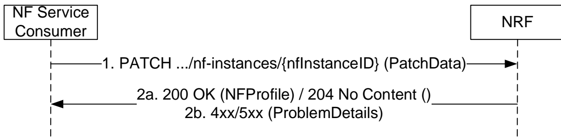
Figure 5.2.2.3.2-1: NF Heart-Beat
