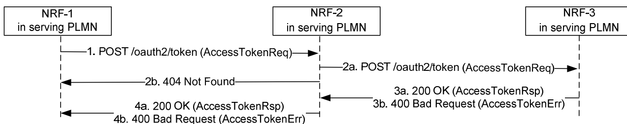
Figure 5.4.2.2.2-1: Access Token Request with intermediate forwarding NRF
