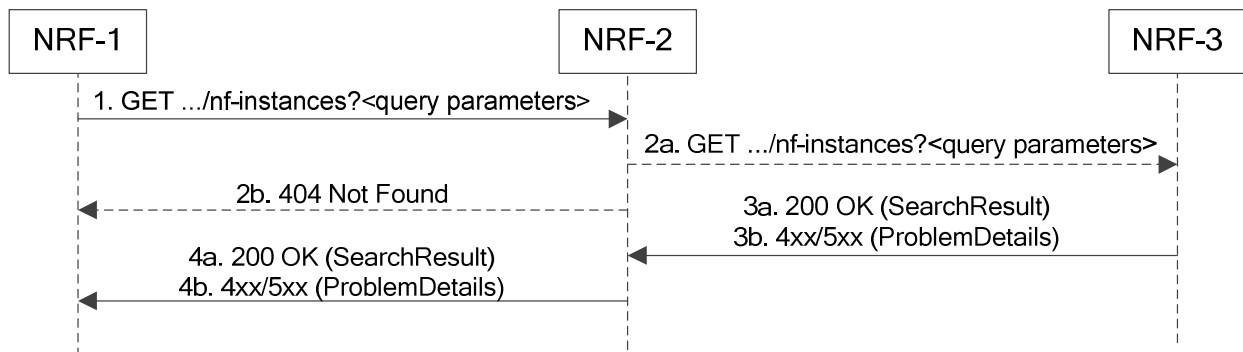
Figure 5.3.2.2.5-1: Service Discovery with intermediate forwarding NRF
