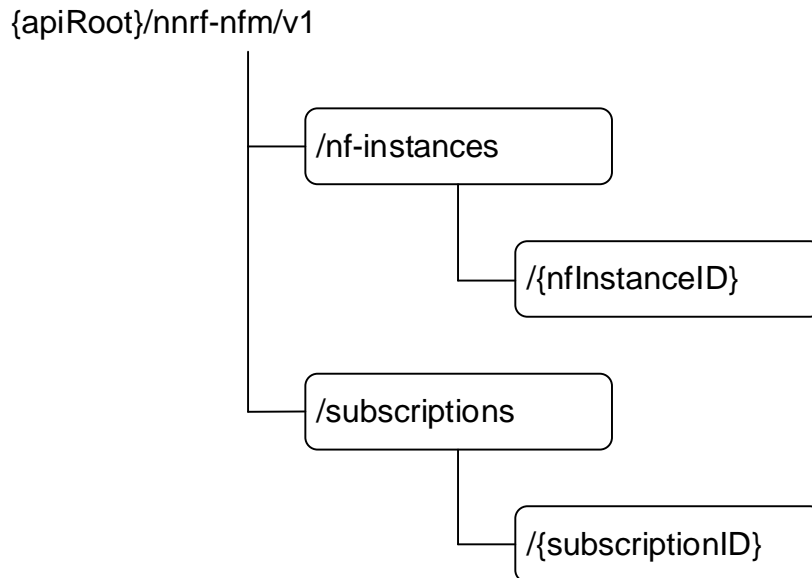
Figure 6.1.3.1-1: Resource URI structure of the NManagement API
