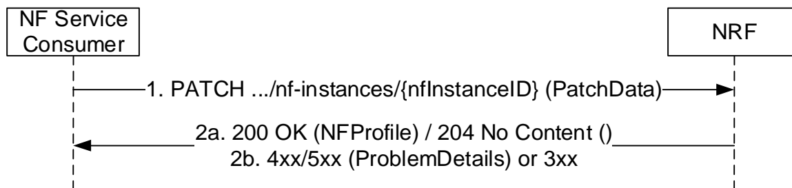
Figure 5.2.2.3.2-1: NF Heart-Beat
