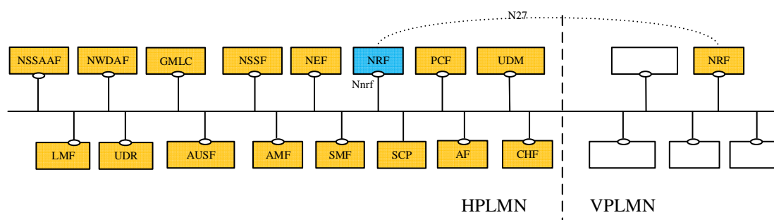
Figure 4-1: 5G System architecture
