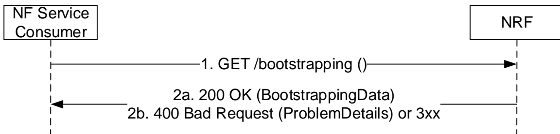
Figure 5.5.2.2.1-1: Bootstrapping Request
