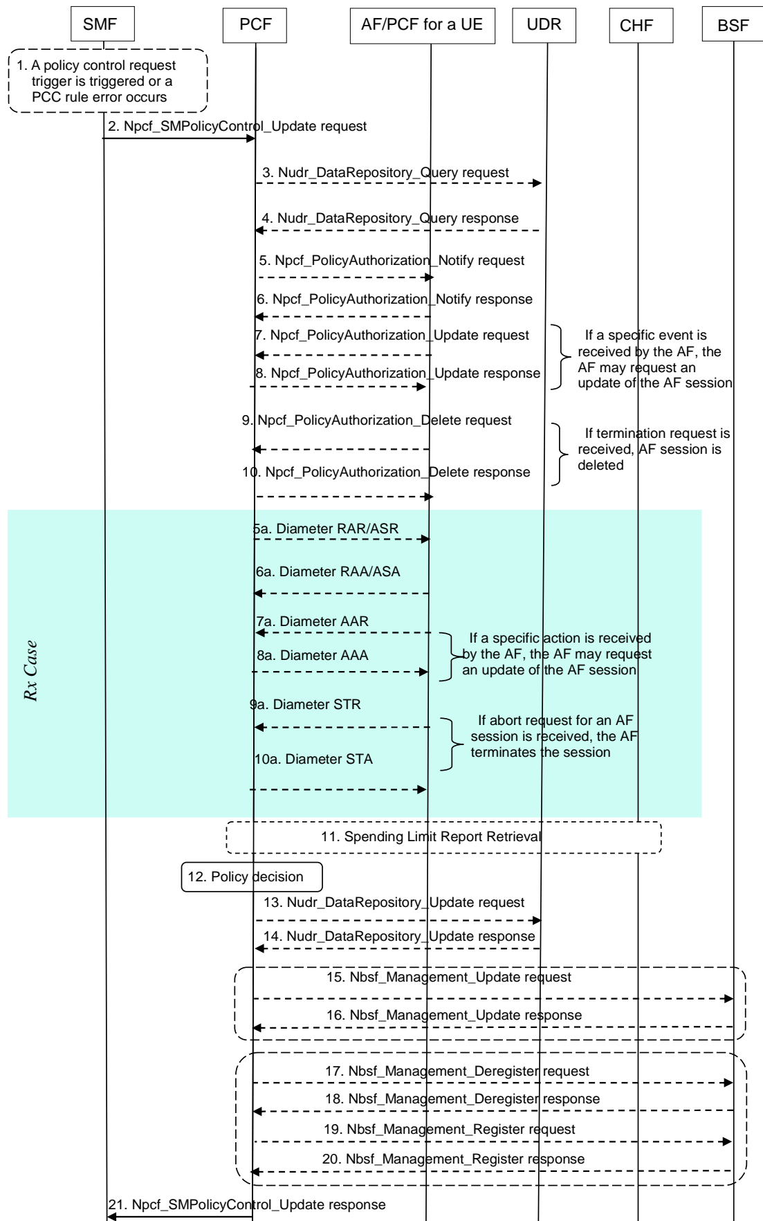
Figure 5.2.2.3-1: SMF-initiated SM Policy Association Modification procedure
