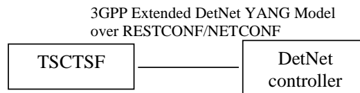
Figure 4.1-5: Interworking between TSCTS and DetNet controller to support Deterministic Networking.
