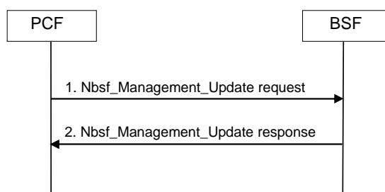
Figure 8.6.3.3-1: Binding information Update procedure
