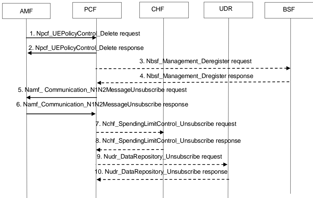
Figure 5.6.3.1.2-1: AMF-initiated UE Policy Association Termination procedure – Non-roaming
