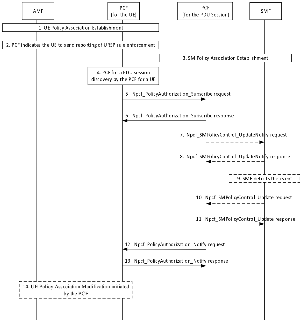
Figure 5.8.2-1: Forwarding of URSP Rule Enforcement Information
