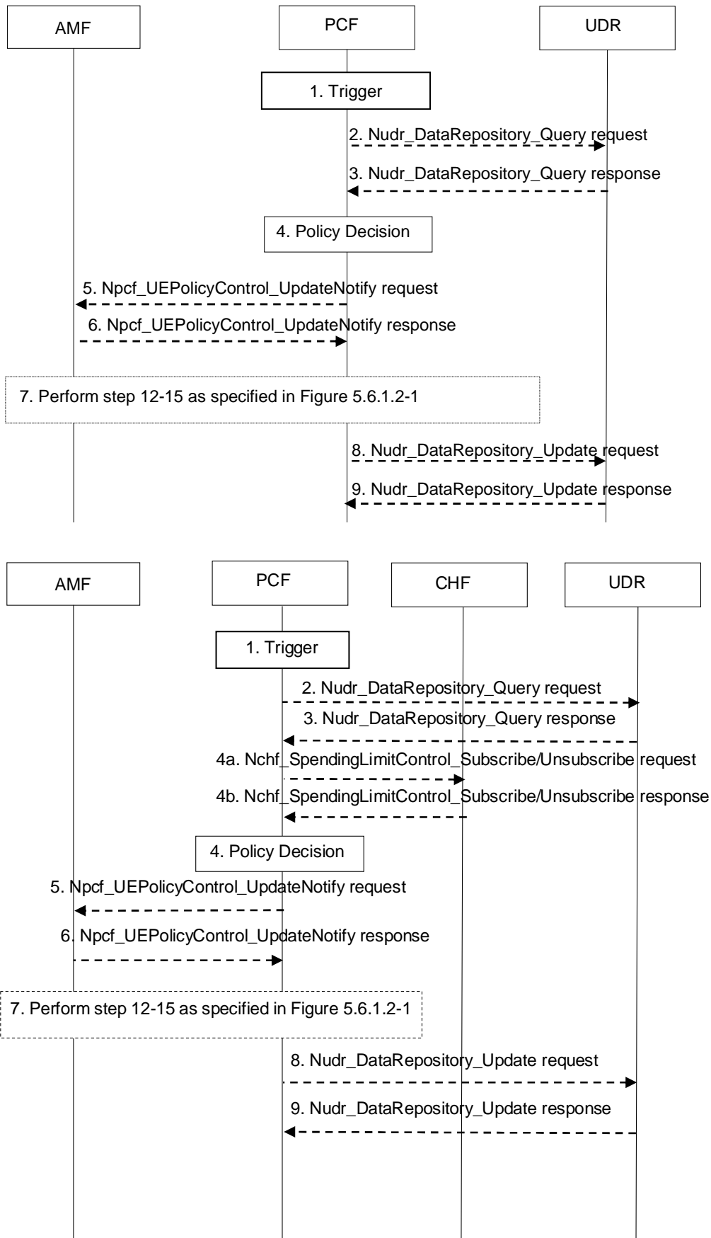
Figure 5.6.2.2.2-1: PCF-initiated UE Policy Association Modification procedure – Non-roaming
