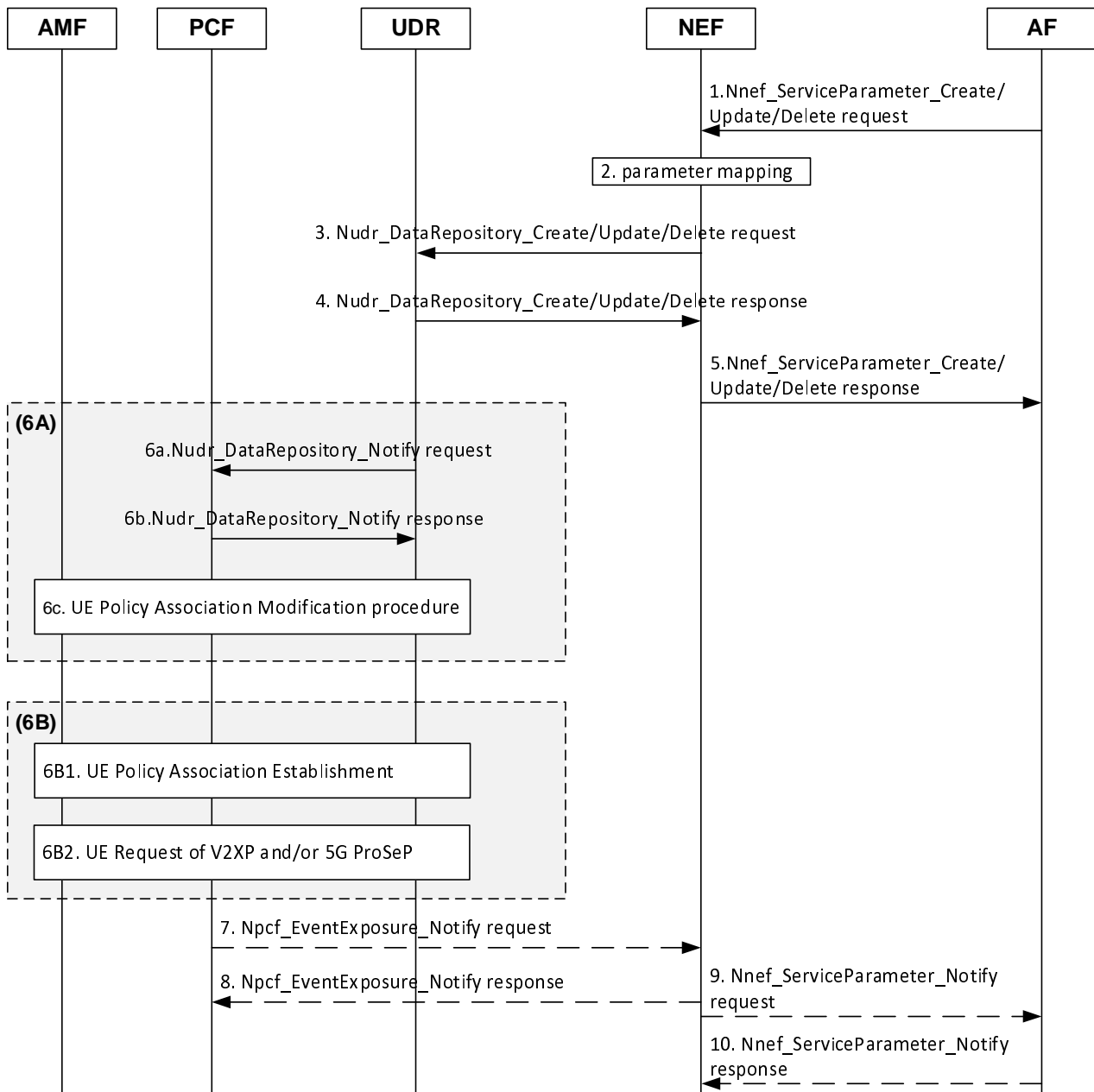
Figure 5.5.8.1-1: AF-based service parameter provisioning procedure to HPLMN
