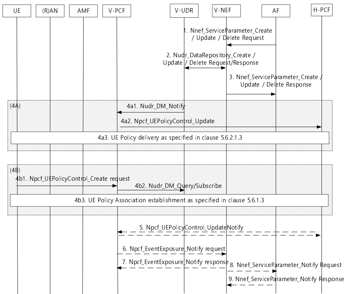
Figure 5.5.8.2-1: AF-based service parameter provisioning procedure to VPLMN
