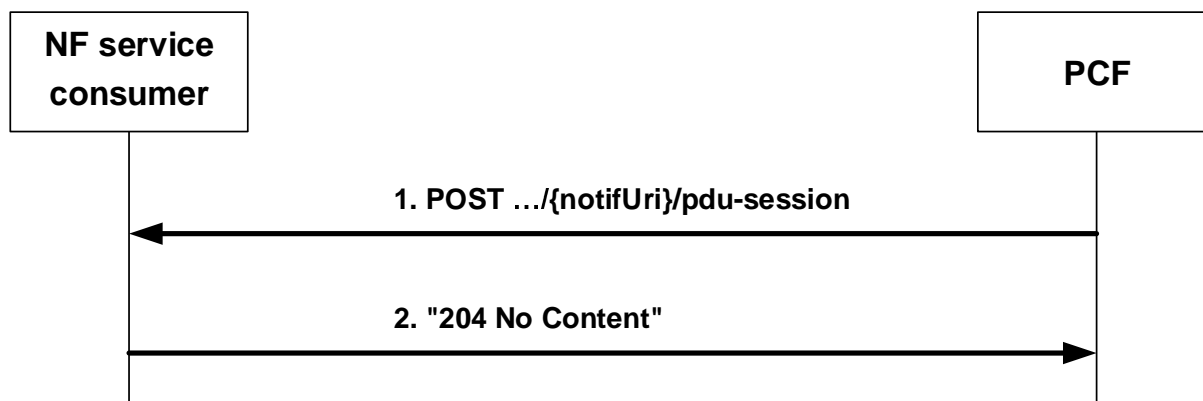
Figure 4.2.5.22-1: Notification about PDU session established/terminated events
