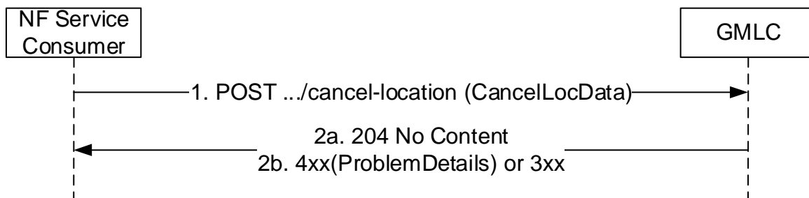
Figure 5.2.2.4.1-1: CancelLocation Request/Response
