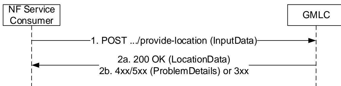
Figure 5.2.2.2-1: ProvideLocation Request/Response for a target UE
