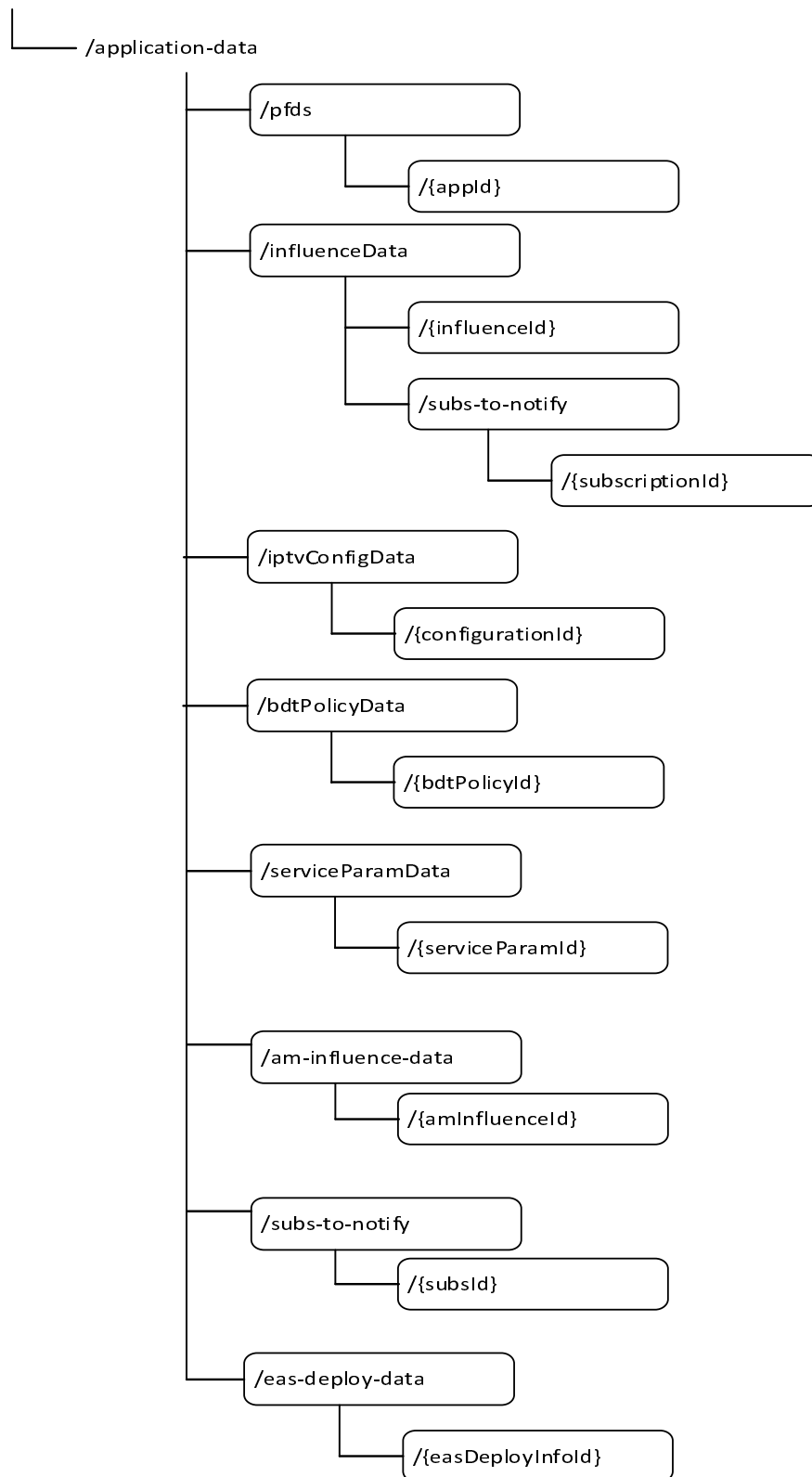
Figure 6.2.2-1: Resource URI structure of the Nudr_DataRepository API for application data
