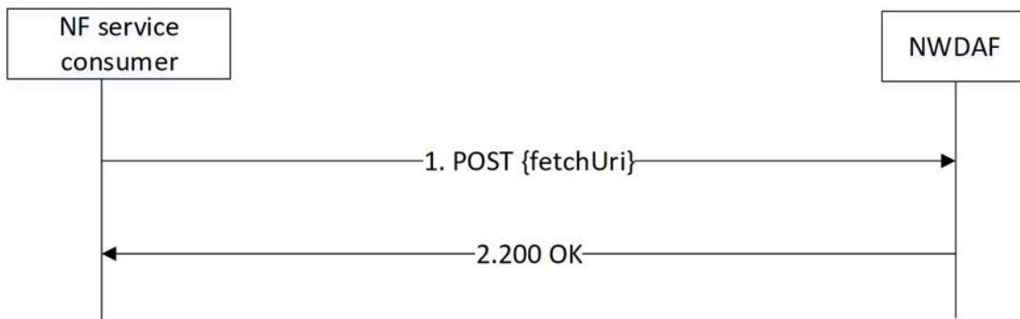
Figure 4.4.2.5.2-1: Requesting to retrieve notified data or analytics
