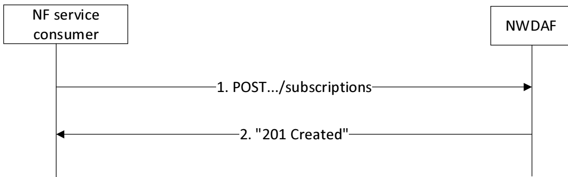
Figure 4.4.2.2-1: NF service consumer subscribes to data or analytics notifications
