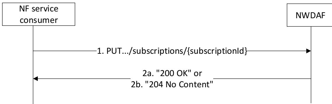
Figure 4.4.2.3-1: NF service consumer updates subscription to data notifications
