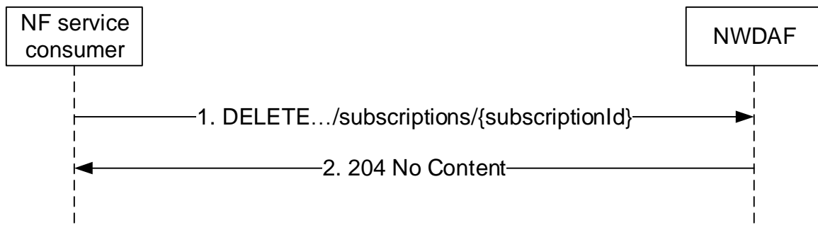
Figure 4.6.2.3.2-1: NF service consumer unsubscribes from notifications
