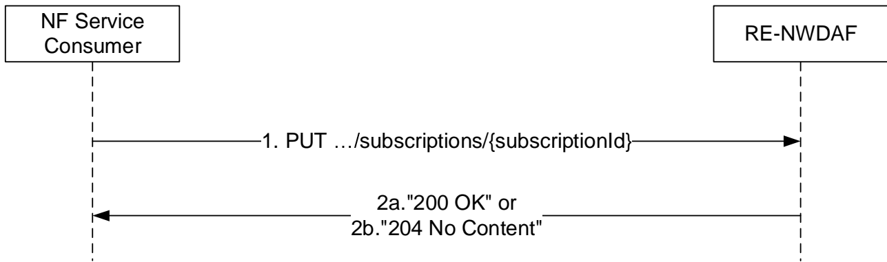
Figure 4.8.2.2.3-1: NF service consumer updates subscription to notifications
