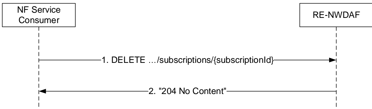
Figure 4.9.2.3.2-1: NF service consumer unsubscribes from notifications
