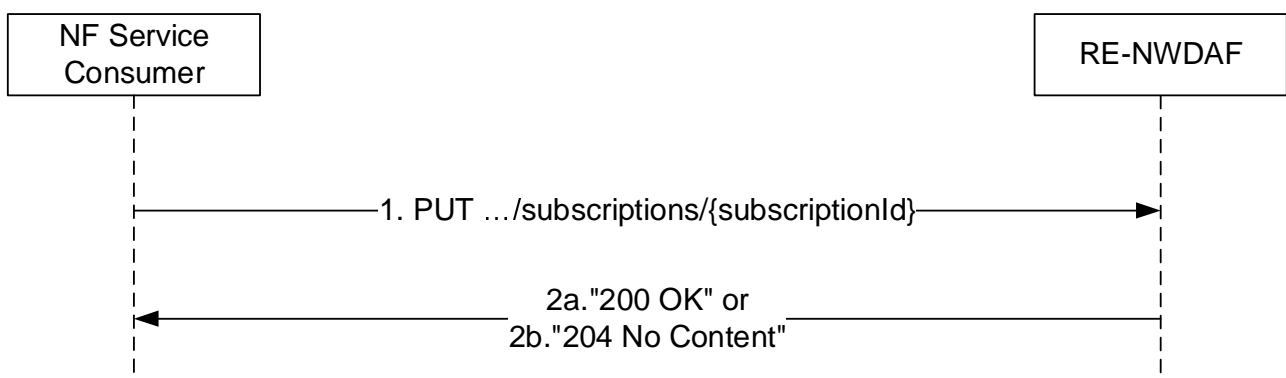
Figure 4.8.2.2.3-1: NF service consumer updates subscription to notifications
