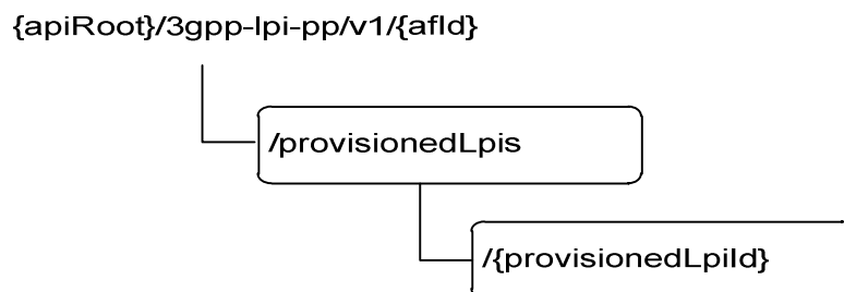
Figure 5.10.1.1-1: Resource URI structure of the LpiParameterProvision API
