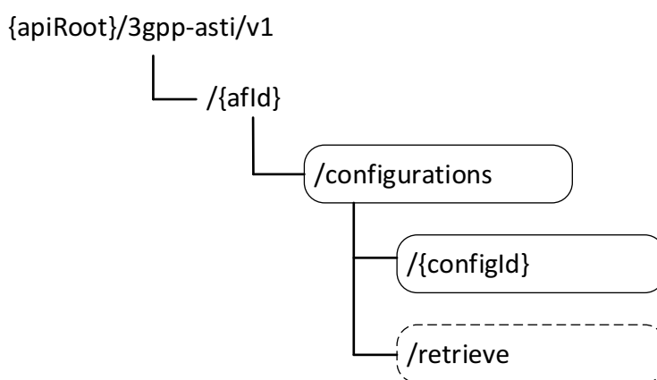
Figure 5.22.1.1-1: Resource URI structure of the ASTI API
