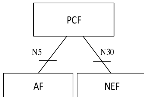
Figure 4.1.2-2: Npcf_EventExposure service Architecture, reference point representation
