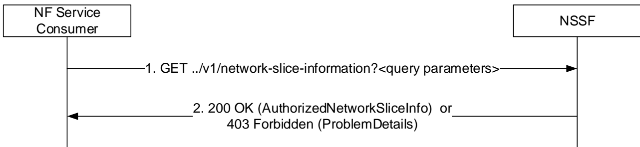
Figure 5.2.2.2-1: Retrieve the network slice information during the registration procedure
