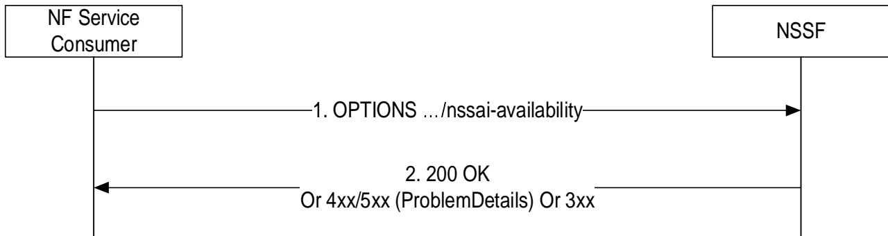
Figure 5.3.2.7.1-1: Procedure for the discovery of communication options supported by the NSSF
