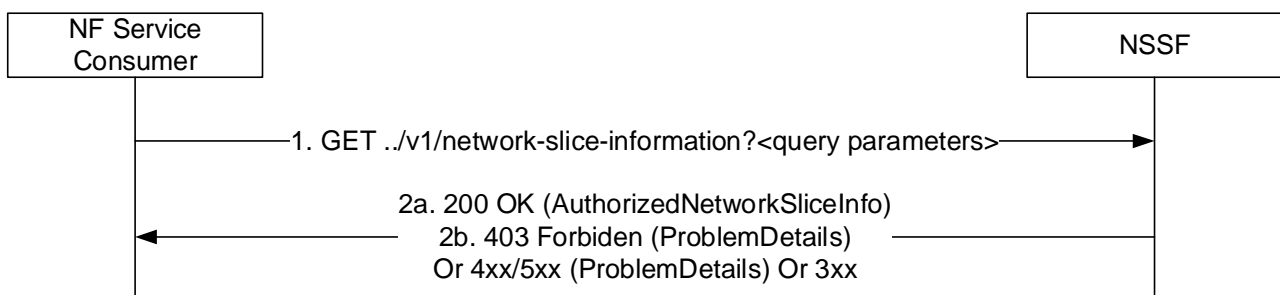
Figure 5.2.2.2.2-1: Retrieve the network slice information during the mobility procedure
