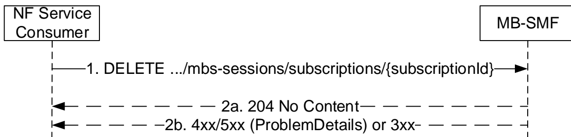
Figure 5.3.2.7.1-1: Unsubscribing from MB-SMF notifications
