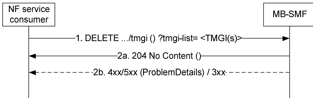
Figure 5.2.2.3.1-1: TMGI deallocation
