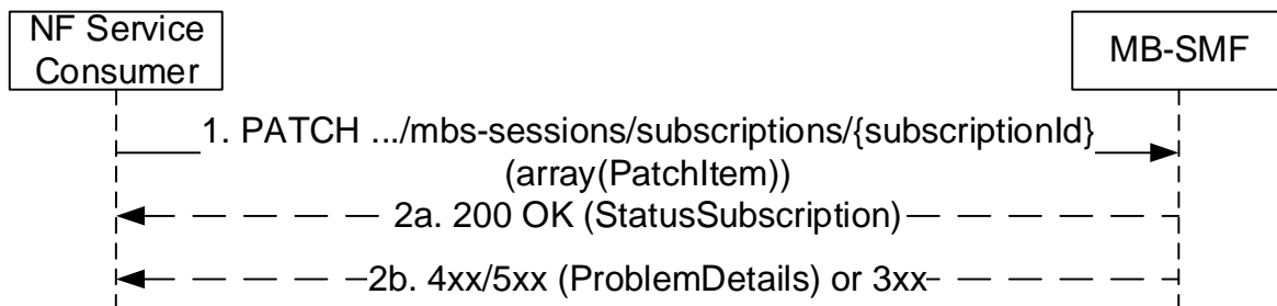
Figure 5.3.2.6.2-1: Updating a subscription to MB-SMF notifications
