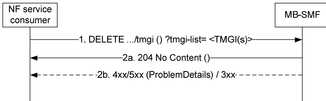
Figure 5.2.2.3.1-1: TMGI deallocation
