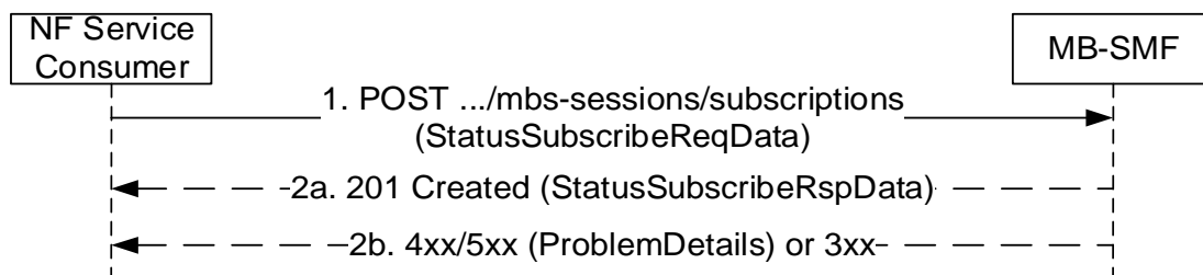
Figure 5.3.2.6.2-1: Subscribing to MB-SMF notifications
