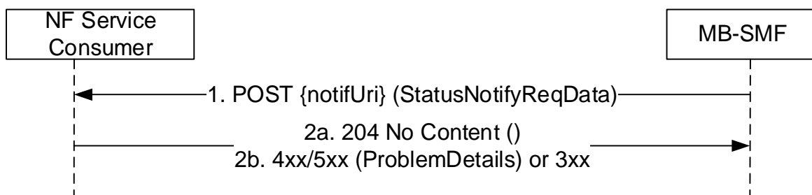
Figure 5.3.2.8.1-1: MB-SMF notifications
