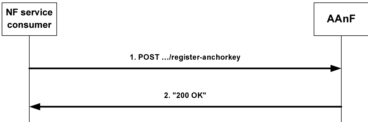
Figure 4.2.2.2-1: Registration of AKMA related key material
