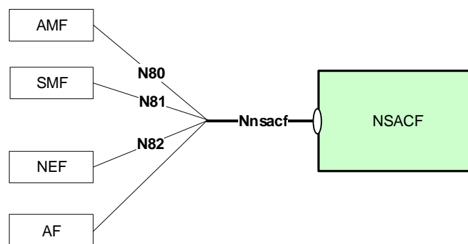
Figure 4-1: Reference model – NSACF
