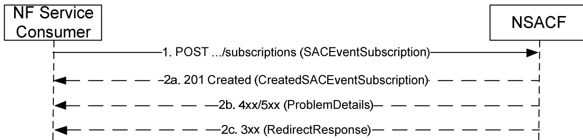
Figure 5.4.2.2-1 Subscribe for Creation
