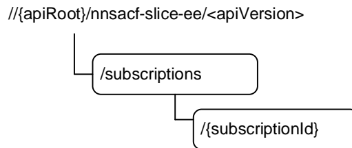
Figure 6.2.3.1-1: Resource URI structure of the Nnsacf_SliceEventExposure API
