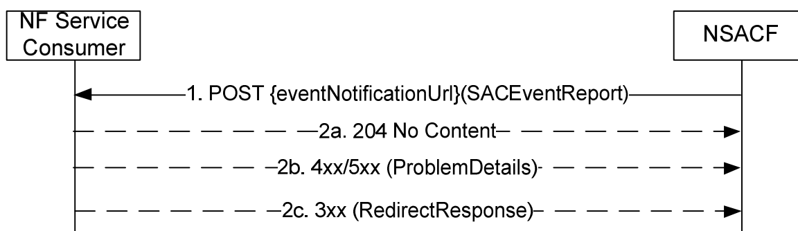
Figure 5.3.2.4.1-1: Notify
