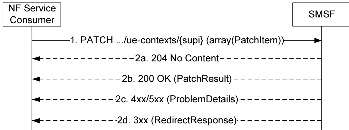
Figure 5.2.2.2.3-1: Modify UE Context in SMSF using HTTP PATCH Method
