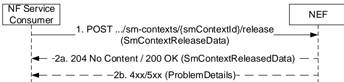
Figure 5.2.2.3.1-1: Delete Service Operation
