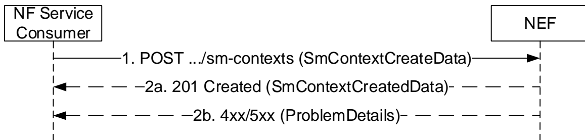
Figure 5.2.2.2.1-1: Create Service Operation
