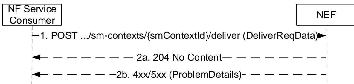
Figure 5.2.2.5.6-1: Deliver Service Operation
