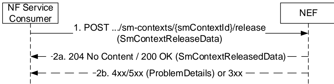
Figure 5.2.2.3.1-1: Delete Service Operation
