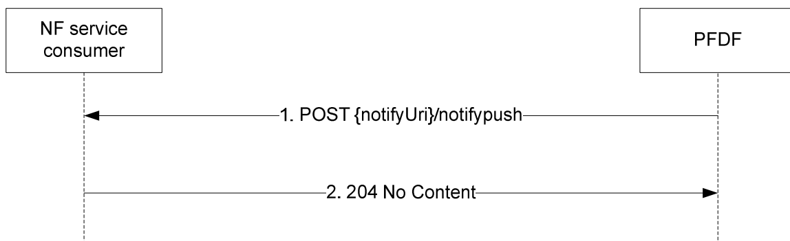
Figure 4.2.4.3-1: Notification PUSH
