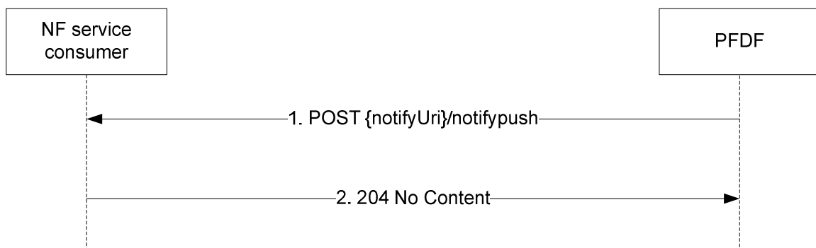
Figure 4.2.4.3-1: Notification PUSH
