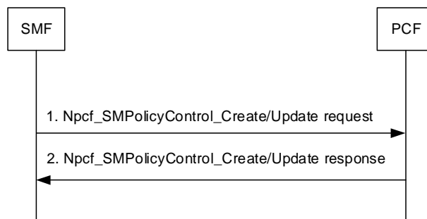
Figure 5.8.4-2: PCF learning from SMF and UPF NWDAFs containing AnLF
