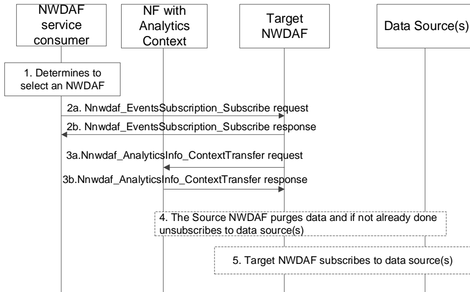
Figure 5.4.1-1: Analytics context transfer initiated by target NWDaf selected by the NWDaf service consumer
