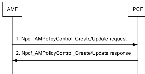
Figure 5.8.4-1: PCF leaning from AMF NWDAFs containing AnLF
