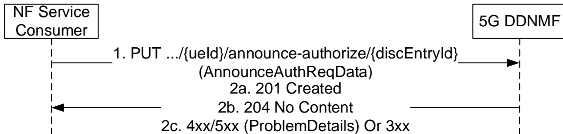
Figure 5.2.2.2-1: Obtain the authorization to announce for a UE
