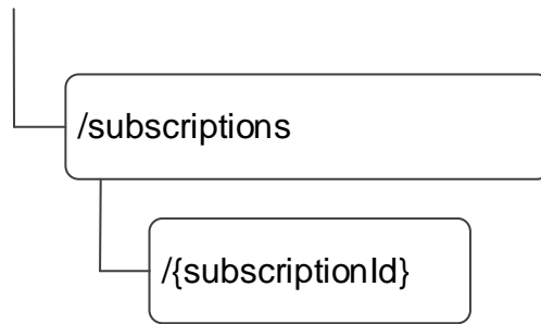
Figure 8.6.2.1-1: Resource URI structure of the Eees_ACRManagementEvent API
