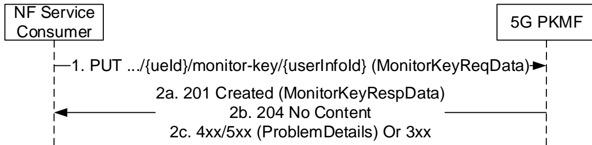
Figure 5.4.2.3.2-1: Monitor Key
