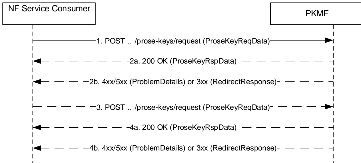
Figure 5.2.2.1-1 ProseKey service operation
