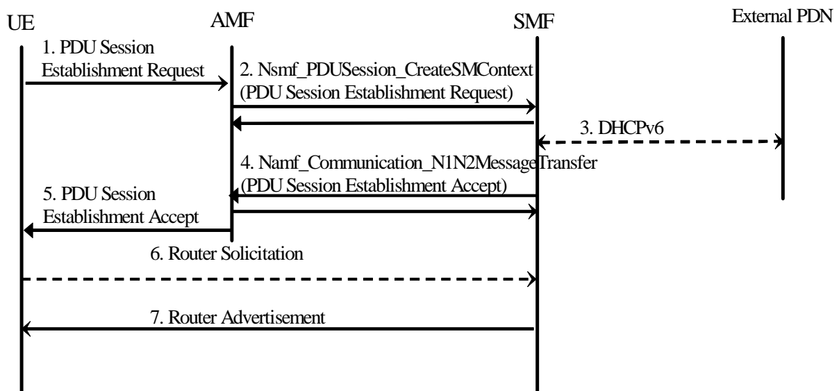
Figure 10.2.3-1: IPv6 Stateless Address Autoconfiguration
