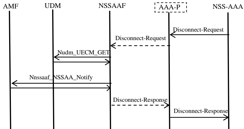
Figure 16.2.2-1: NSS-AAA initiated revocation of network slice authorization with RADIUS
