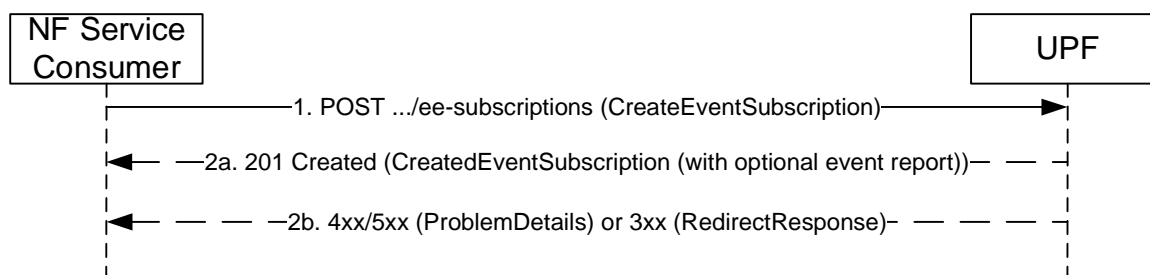
Figure 5.2.2.2-1 Subscription creation
