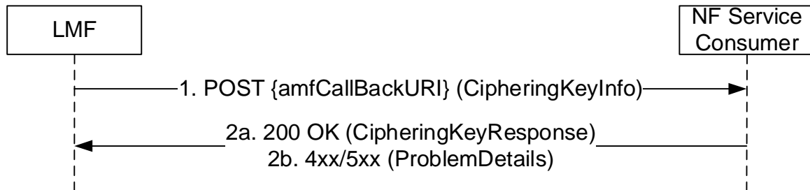
Figure 5.3.2.2.3-1: CipheringKeyData Notify
