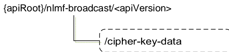
Figure 6.2.3.1-1: Resource URI structure of the Nlmf_Broadcast API Table 6.2.3.1-1 provides an overview of the resources and applicable HTTP methods.
