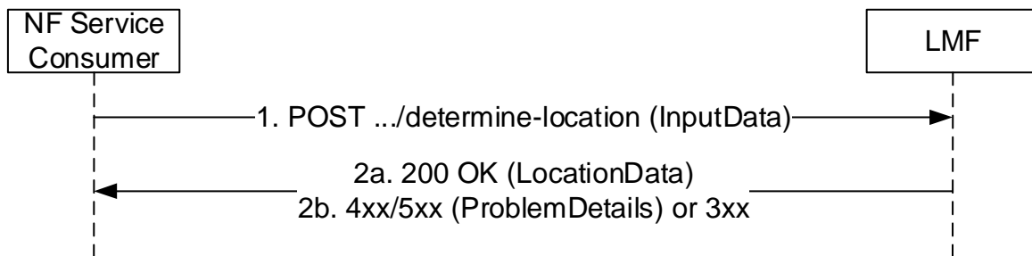
Figure 5.2.2.2-1: DetermineLocation Request
