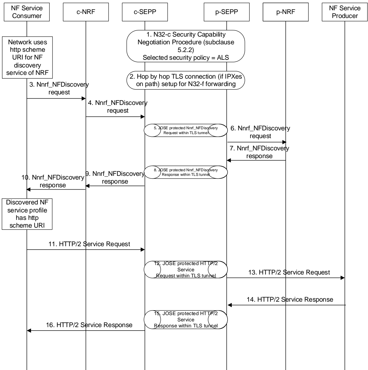
Figure C.3.1-1 End to end call flow when http scheme URI is used and ALS security is used between SEPPs
