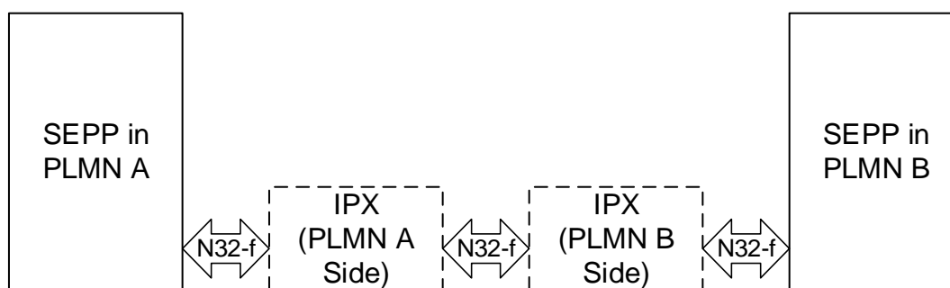
Figure 4.2.3-1: N32-f Interface
