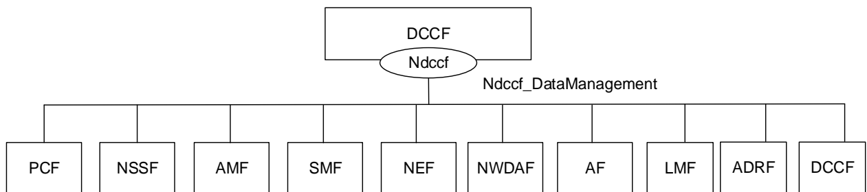
Figure 4.2.1.2-1: Ndcf_DataManagement service architecture, SBI representation
