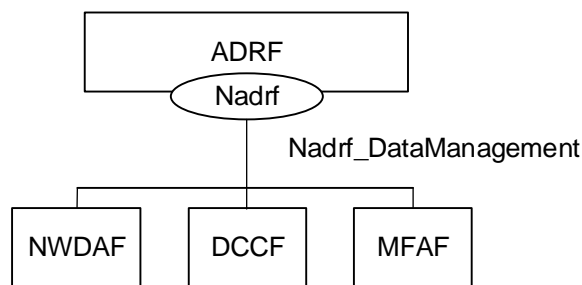
Figure 4.2.1.2-1: Reference Architecture for the Ndrf_DataManagement Service; SBI representation
