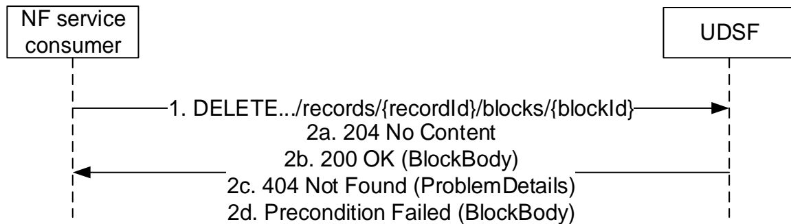
Figure 5.2.2.5.3-1: Delete a block
