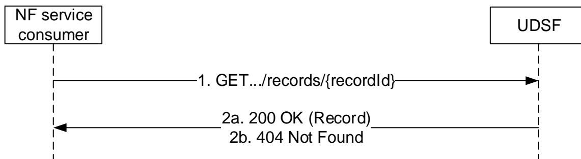
Figure 5.2.2.2.2-1: Requesting a Record
