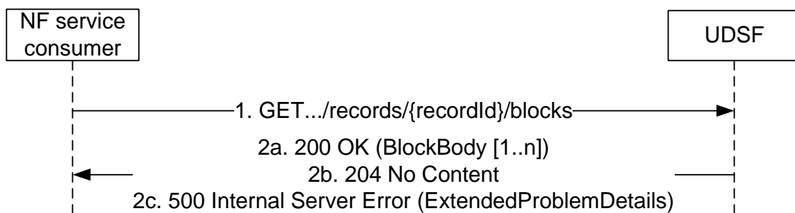
Figure 5.2.2.2.4-1: Requesting Blocks
