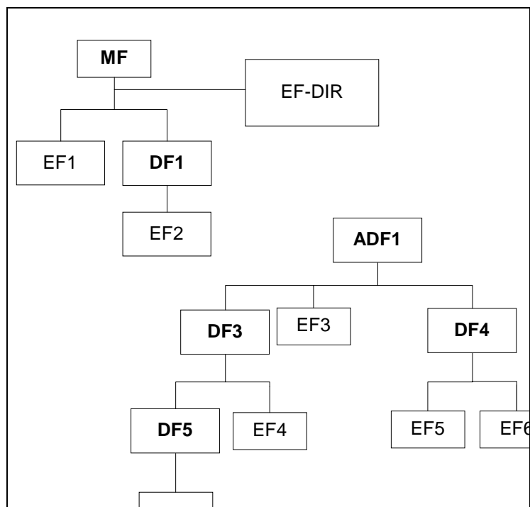
Figure 8.4: Example of a logical structure
