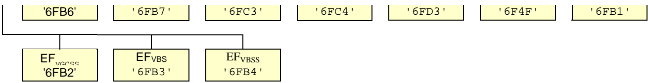
Figure 4.2: File identifiers and directory structures of USIM
